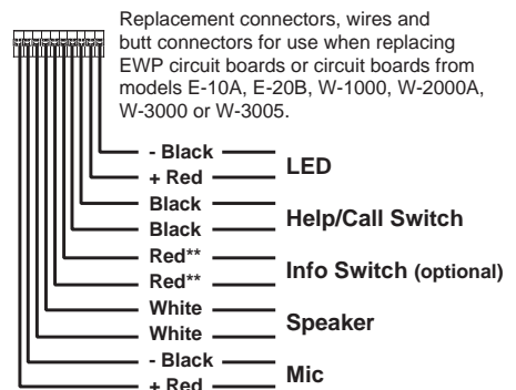
FIGURE 1 Replacement Cable Assembly (included)
